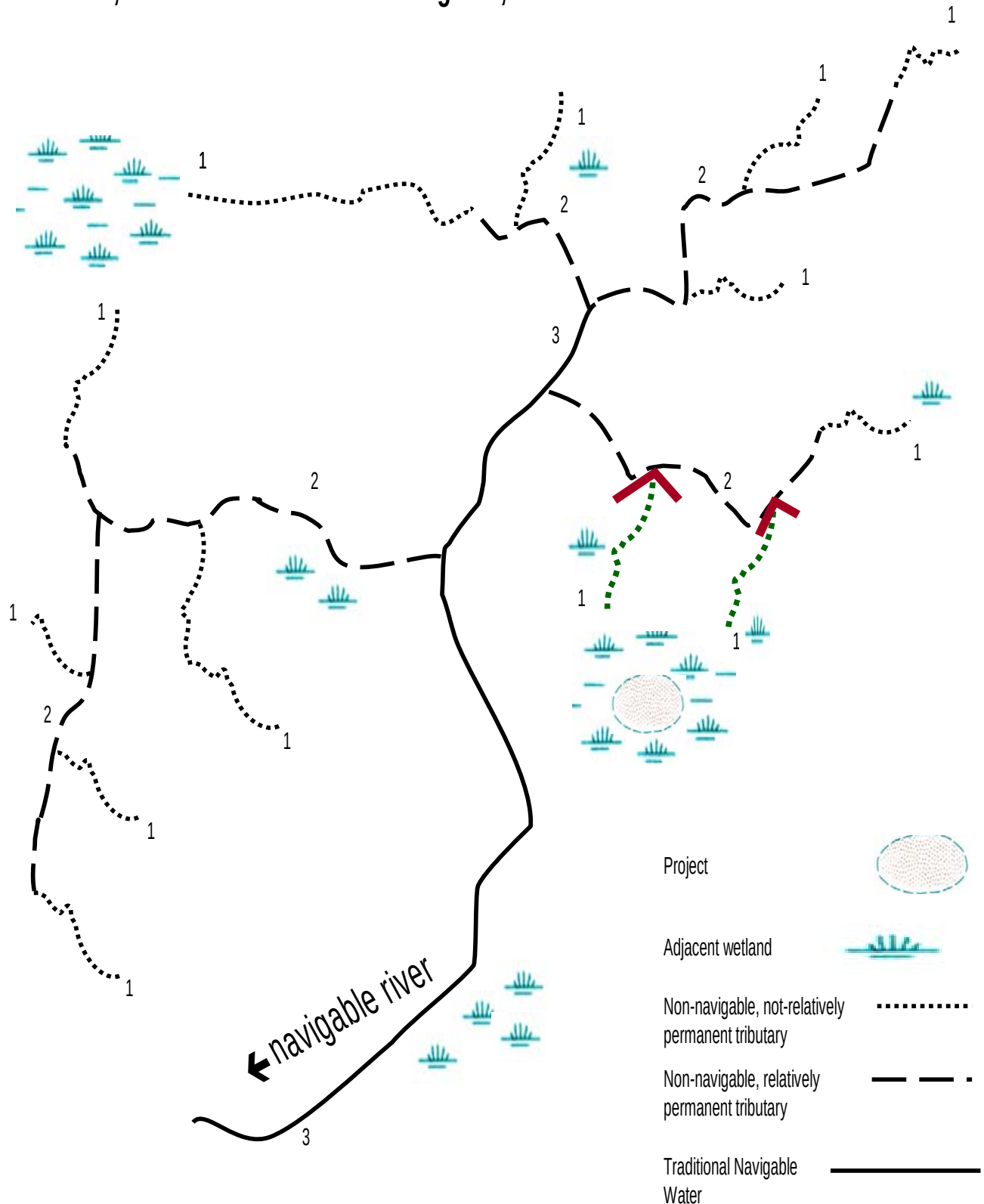
Illustration 5: Project involves a wetland adjacent to two tributaries with non-RPWs. The “relevant reach” includes the wetland, and any other wetlands adjacent to those tributaries, and both tributaries colored green; the reach terminates at the red lines.
