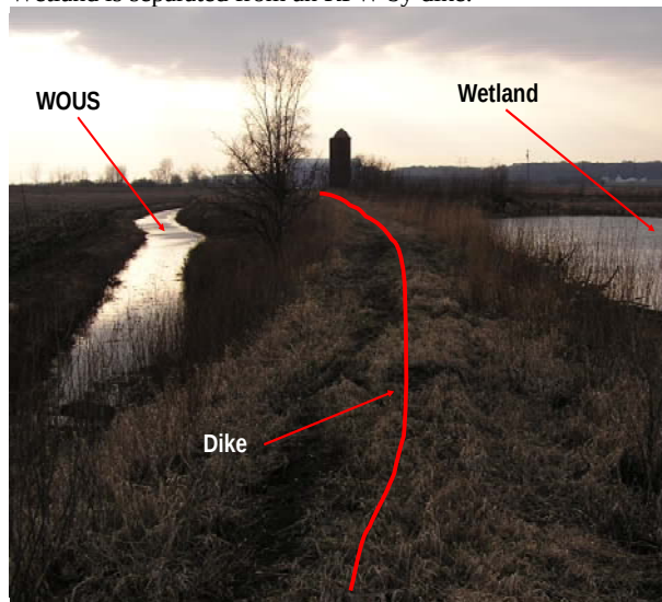
Photo 34. Non-abutting wetland, IL. Wetland is separated from an RPW by dike.
